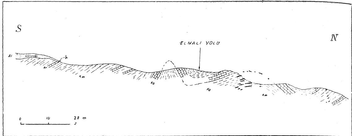
Fig. 2 « Section of Toprakpınar stream, near Düğer
