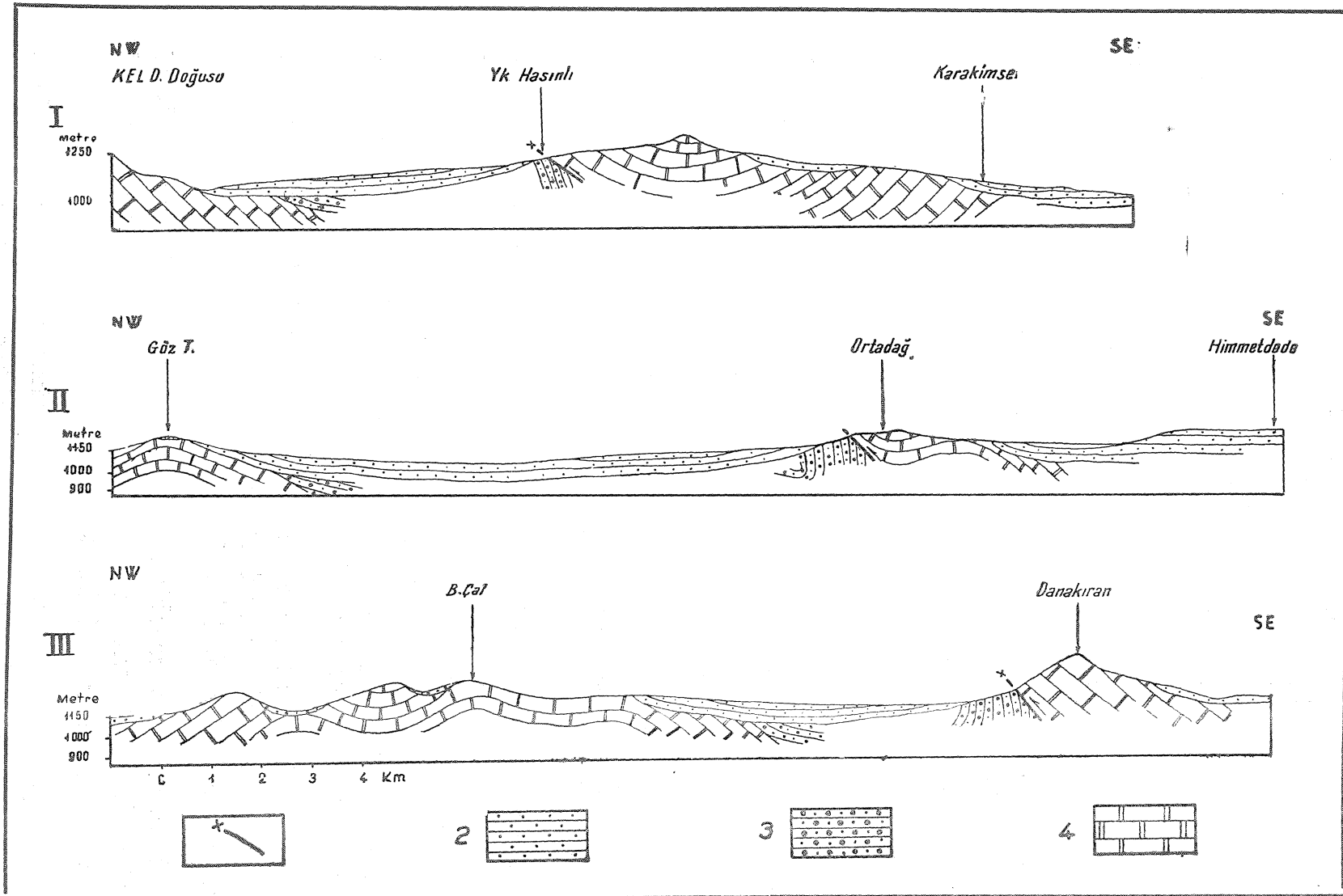
Fig. 1 - Geological section of the Himmetdede Area
